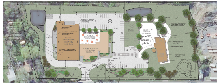
Colored Site Plan - Prison City Brewing
